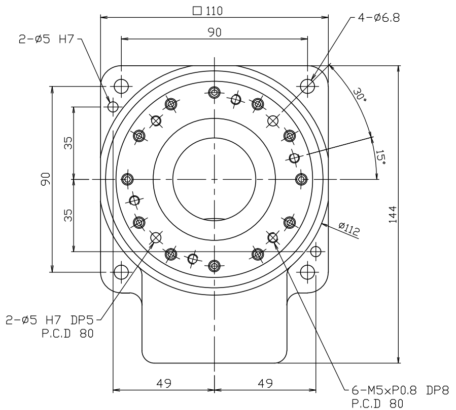
[ CROSSED ROLLER BEARING ]
